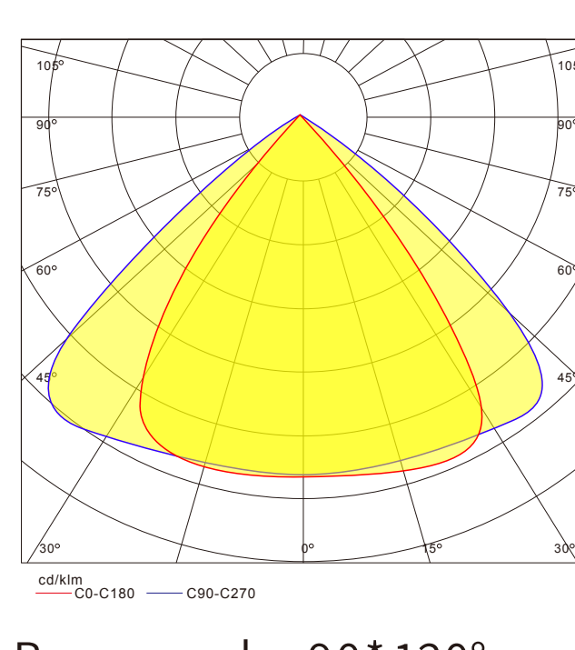
Beam angle: 90°120°
